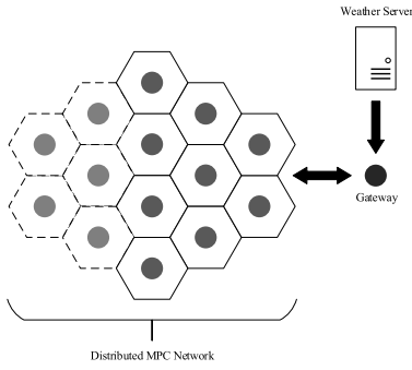
Fig. 2. The structure of the proposed CPS for the optimal heating-cooling of building.
