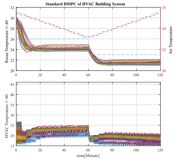
Fig. 10. Temperature regulation response of the case study building for the cooling mode when the distributed standard MPC of [4] and [7] is used. To figure illustrates large steady state error around the desired set points of 26 Centigrade and 23 Centigrade.
