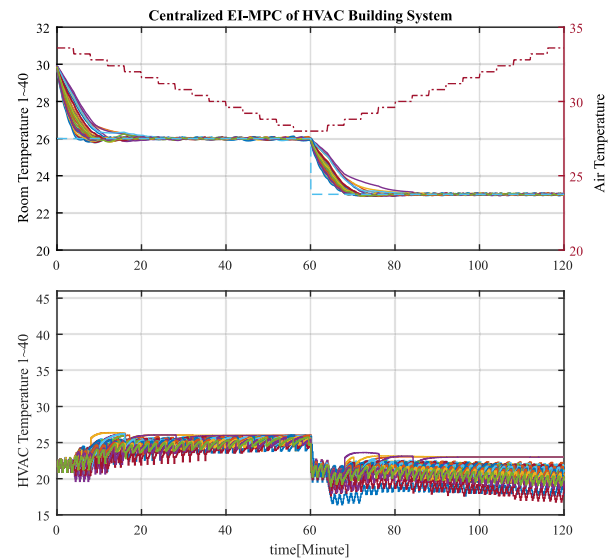
Fig. 9. Temperature regulation response of the case study building for the cooling mode when the centralized EI-MPC is used. Different colors are used for different rooms. Top figure illustrates that the temperature of each room reaches to the desired temperature. Bottom figure illustrates control efforts for such a good temperature regulation.
