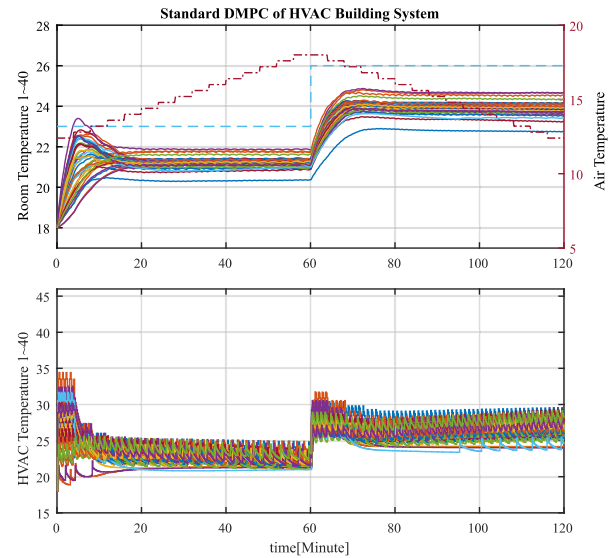
Fig. 6. Temperature regulation response of the case study building for the heating mode when the distributed standard MPC of [4] and [7] is used. Top figure illustrates large steady state error in temperature regulation around the desired set points of 23 Centigrade and 26 Centigrade.
