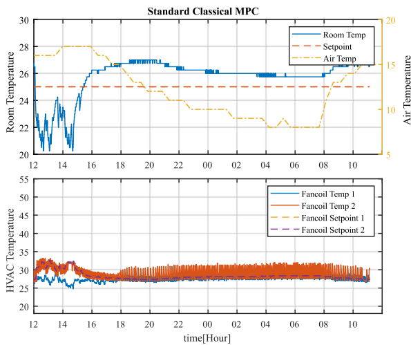
Fig. 18. Room temperature regulation response when the distributed MPC proposed in [4], [7] is used.
