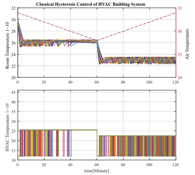
Fig. 12. Temperature regulation response of the case study building for the cooling mode when the traditional hysteresis-based method is used. Top figure illustrates that there are high fluctuation ( \pm 1 Centigrade) around the desired set points of 26 Centigrade and 23 Centigrade. Bottom figure illustrates that the temperatures of the fan-coil units are frequently changing between 25 Centigrade and 12 Centigrade.
