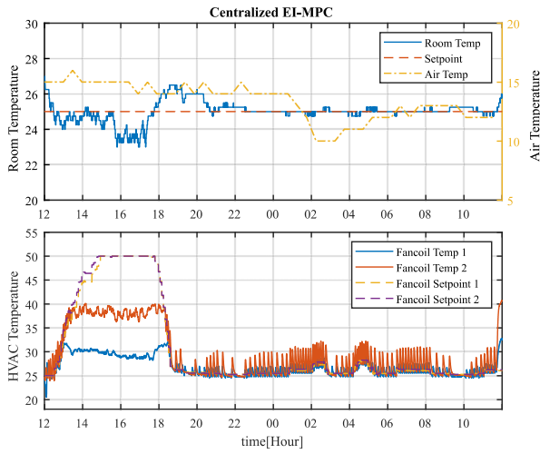
Fig. 16. Room temperature regulation response when the centralized EI-MPC is used.
