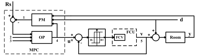
Fig. 3. The block diagram of the proposed control strategy in each room. 1: Predicted Output, 2: Constraints, 3: Cost Functions, 4: Predicted Input, 5: Fan-Coil Air Temperature, PM: Plant Model, OP: Optimizer.
