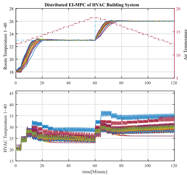
Fig. 7. Temperature regulation response of the case study building for the heating mode when the proposed distributed EI-MPC is used. Top figure illustrates that the temperature of each room reaches to the desired temperature. Bottom figure illustrates similar control efforts as the centralized EI-MPC.
