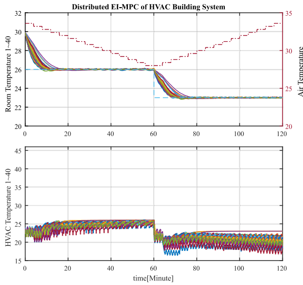
Fig. 11. Temperature regulation response of the case study building for the cooling mode when the proposed distributed EI-MPC is used. Top figure illustrates that the temperature of each room reaches to the desired temperature. Bottom figure illustrates similar control efforts as the centralized EI-MPC.
