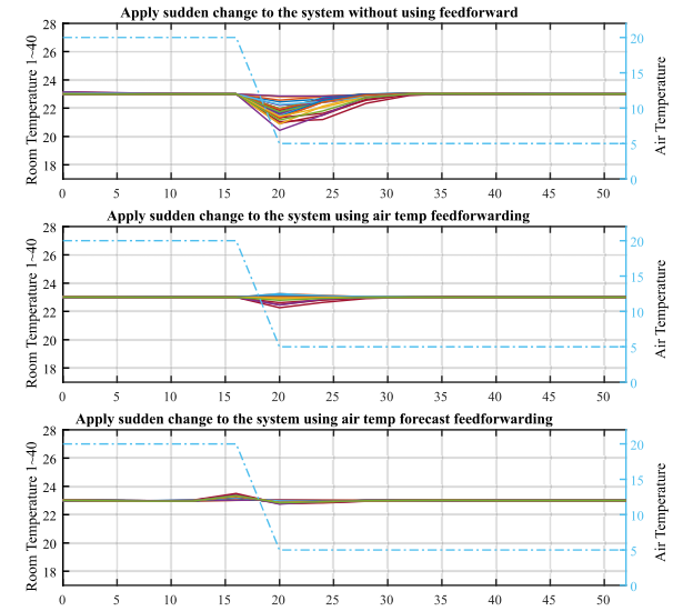
Fig. 13. The effects of not using/using feed-forward mechanism for the rooms temperature regulation. Top figure: without outside (air) temperature feed-forward mechanism. Middle figure: with air temperature feed forwarding. Bottom figure: with air temperature forecast feed forwarding.
