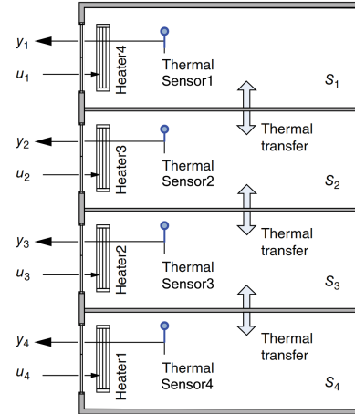
Fig. 1. The multi-zone building temperature control system [1].
