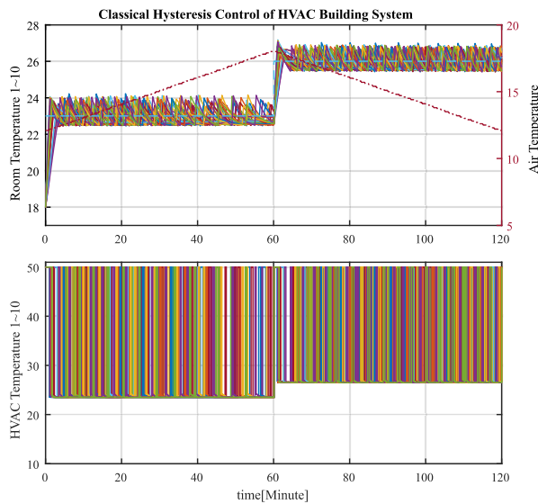
Fig. 8. Temperature regulation response of the case study building for the heating mode when the traditional hysteresis - based method is used. Different colors are used for different rooms. Top figure illustrates that there are high fluctuation ( \pm 1 Centigrade) around the desired set points of 23 Centigrade and 26 Centigrade. Bottom figure illustrates that the temperature of the fan-coil units are frequently changing between 24 Centigrade and 50 Centigrade.
