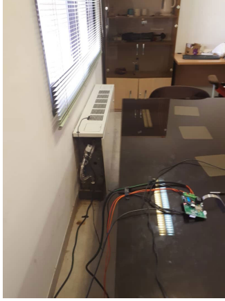
Fig. 15. A view of the room equipped with smart thermostats.
