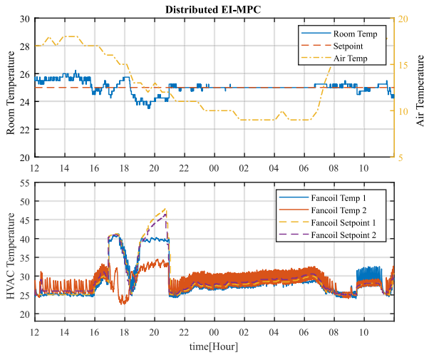
Fig. 17. Room temperature regulation response when the distributed EI-MPC is used.
