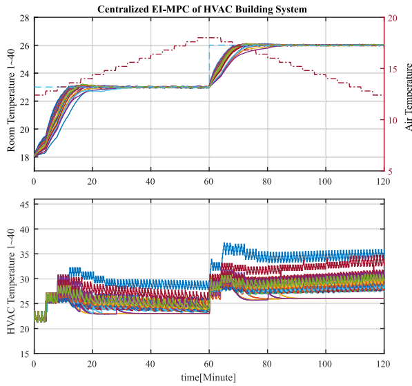
Fig. 5. Temperature regulation response of the case study building for the heating mode when the centralized EI-MPC is used. Different colors are used for different rooms. Top figure illustrates that the temperature of each room reaches to the desired temperature. Bottom figure illustrates control efforts.
