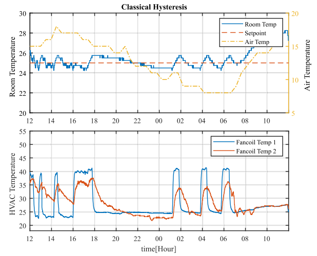
Fig. 19. Room temperature regulation response when the available hysteresis-based control method is used.
